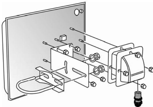
Figure 1-2. Attaching the Boot Cover to the TR-WMX-3.5
