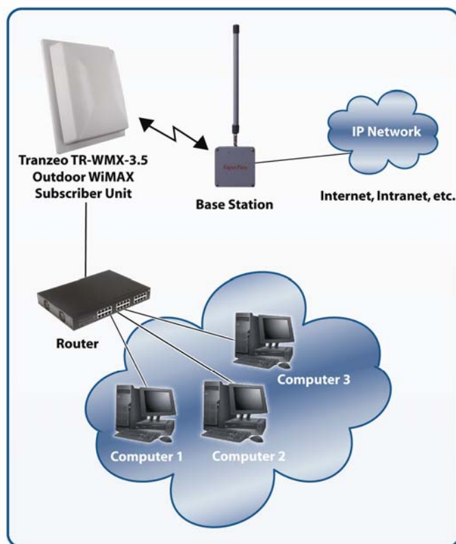
Figure 1-1. Example of a TR-WMX-3.5 Configuration
