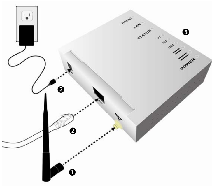
Figure 1-4. Installing the Indoor Unit
