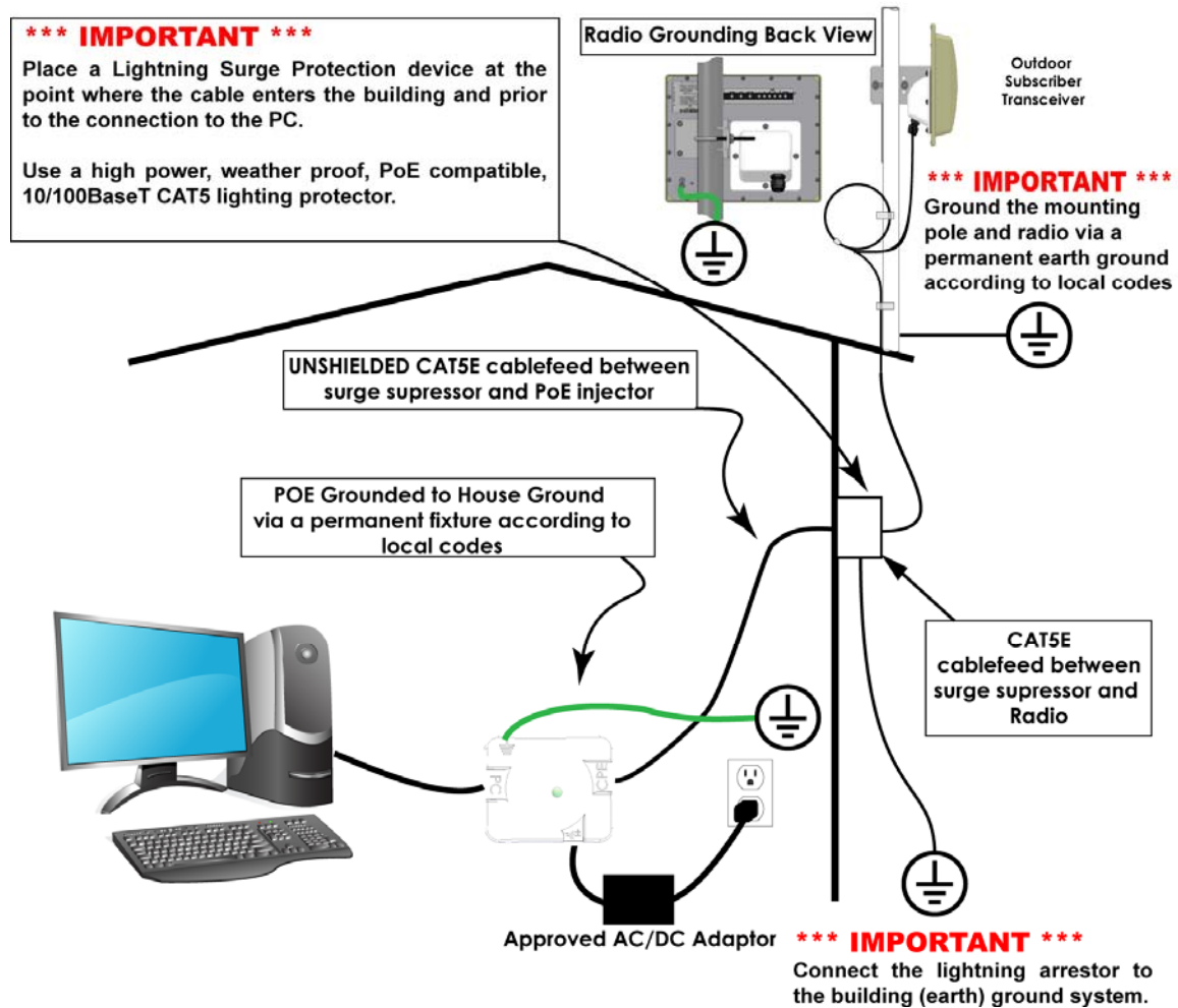
Figure 1-3. Sample TR-WMX-3.5 Installation
